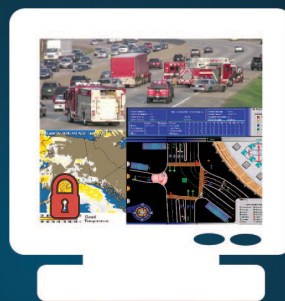
Operator Desktops
