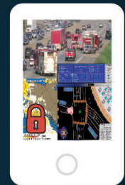
Mobile Devices
